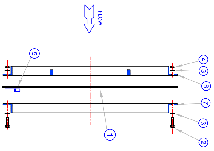
TYPICAL VIEW OF FRAME ARRANGEMENT (FOR ALTERNATIVE FRAME OPTIONS SEE SHT 99)
