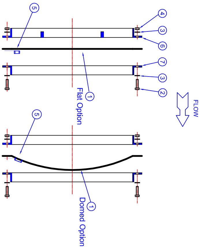
TYPICAL VIEW OF FRAME ARRANGEMENT (FOR ALTERNATIVE FRAME OPTIONS SEE SHT 99)
