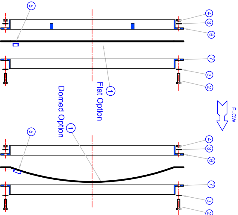
TYPICAL VIEW OF FRAME ARRANGEMENT (FOR ALTERNATIVE FRAME OPTIONS SEE SHT 99)
